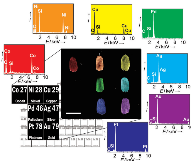
Figure 1. SEM element mapping images of seven metallic wing-scale replicas. All of the metallic replicas were imaged under high vacuum without metal sputtering that was needed for original nonconductive butterfly scale samples. Silicon signals originate from the Si wafer substrate, and slight oxidation occurs for the Co and Ni replicas (in the Supporting Information it is also mentioned that Cu is slightly oxidized). Au NPs as catalysts could not be identified in the replicas (except for the Au scale) owing to their small numbers in comparison with grains in the continuous deposited metal layers. Pseudo colors based on mapping data were generated directly using the software Microanalysis Suite (18d + SPS, Oxford Instruments Inca). Scale bar: 50 \mu\text{m} .
